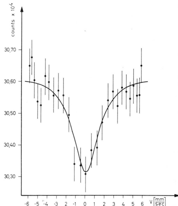
Fig. 1. Mössbauer spectrum of the 104 \text{ keV} transition of ^{180}\text{W} at 20^\circ\text{K} .
